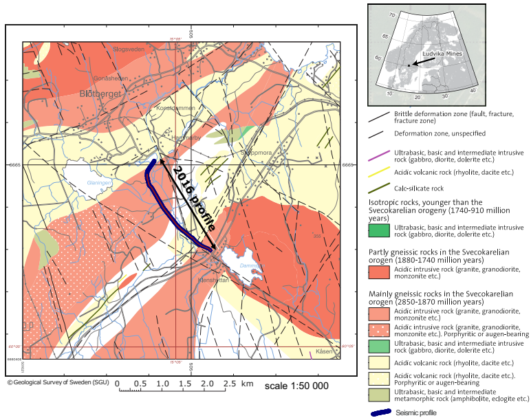
Figure 5.6: Bedrock map of the Blötberget mine and the location of the seismic profile, focus of this study, modified from the Geological Survey of Sweden.
