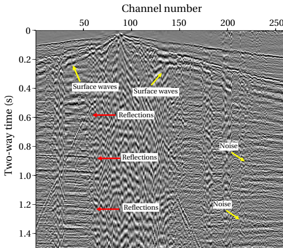
Figure 3.6: The same common-shot gather as in Figure 3.4, after the application of f-k filtering for surface-wave suppression. Band-pass filtering to remove some low-frequency noises and AGC were applied for plotting. The red arrows point to reflection arrivals, the yellow arrows point to surface-wave arrivals and other noises present in the common-shot gather.
