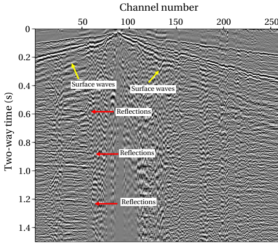
Figure 3.5: The same common-shot gather as in Figure 3.4, after interferometric surface-wave suppression. Band-pass filtering to remove some low-frequency noises and AGC were applied for plotting. The red arrows point to reflection arrivals, the yellow arrows point to surface-wave arrivals and other noises present in the common-shot gather.
