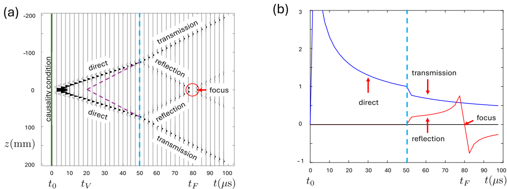
Figure 2. (a) Cross-sections at x = 0 of the Green's function of figure 1, i.e. \mathcal{G}(\mathbf{x}, \mathbf{O}, t, 0)|_{x=0} . (b) Scaled amplitude cross-sections of (a), measured along the direct and transmitted waves (blue) and along the reflected wave (red).
