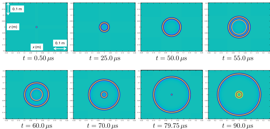
Figure 1. Snapshots of the Green's function \mathcal{G}(\mathbf{x}, \mathbf{O}, t, 0) (convolved with a spatial wavelet) for a piecewise constant time-dependent material, with a time boundary at t = 50.0 \mu\text{s} (see also electronic supplementary material, movie Green.mp4 in the online material).
